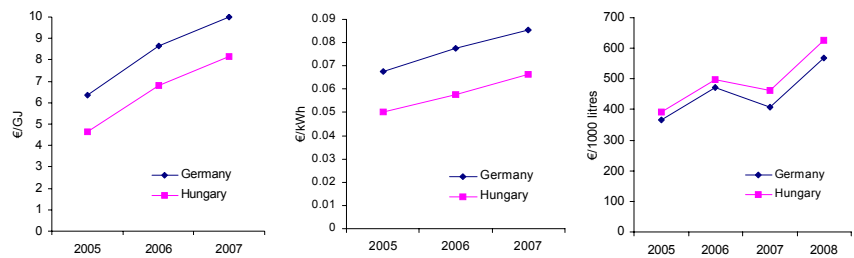
A-Figure 2 Energy product prices; (a) and (b) for large industrial stadard consumers.
